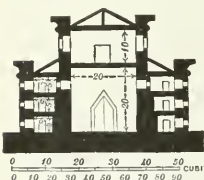
FIG. 2. ELEVATION OF THE TEMPLE OF SOLOMON IN A-B OF PLAN
