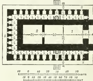
FIG. 1. PLAN OF THE TEMPLE OF SOLOMON
