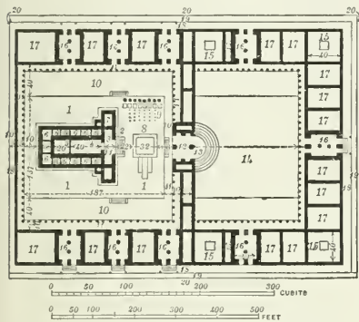
FIG. 3. PLAN OF THE TEMPLE OF HEROD
